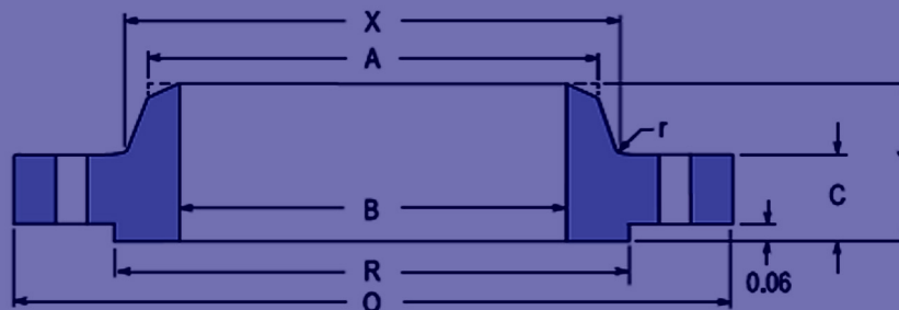
WELDING NECK
