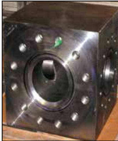
7 1/16" 5M Studded Tee
