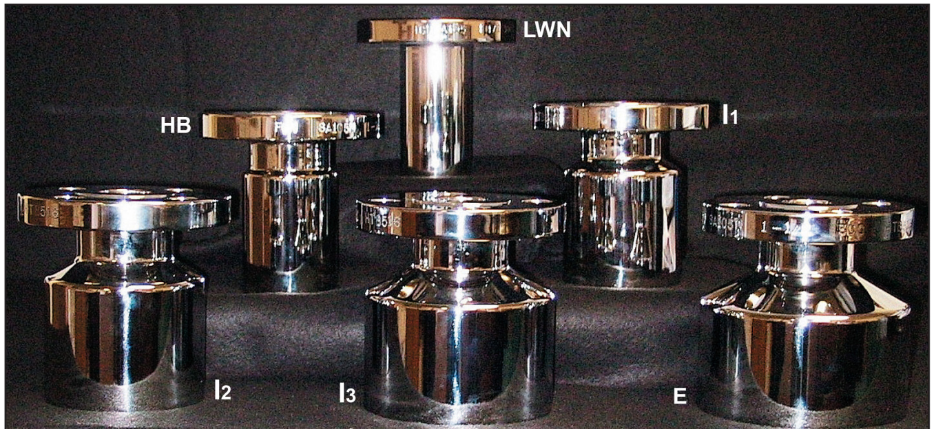
Standard Integral Forged Pressure Vessel Connections
