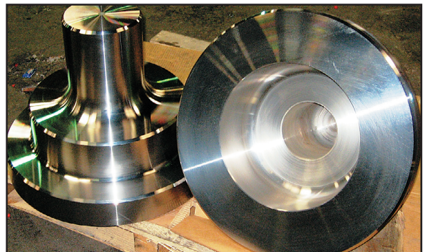
Completed Double Hubbed Flanged Bonnet
