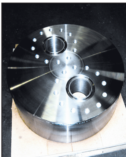
Dual Adapter 7 1/16" 10M x 7 1/16" 10M
