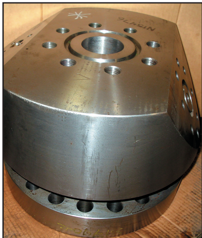
Tubing Bonnet 11" 5M x 4" 5M with 2" 5M Outlet and Control Line
